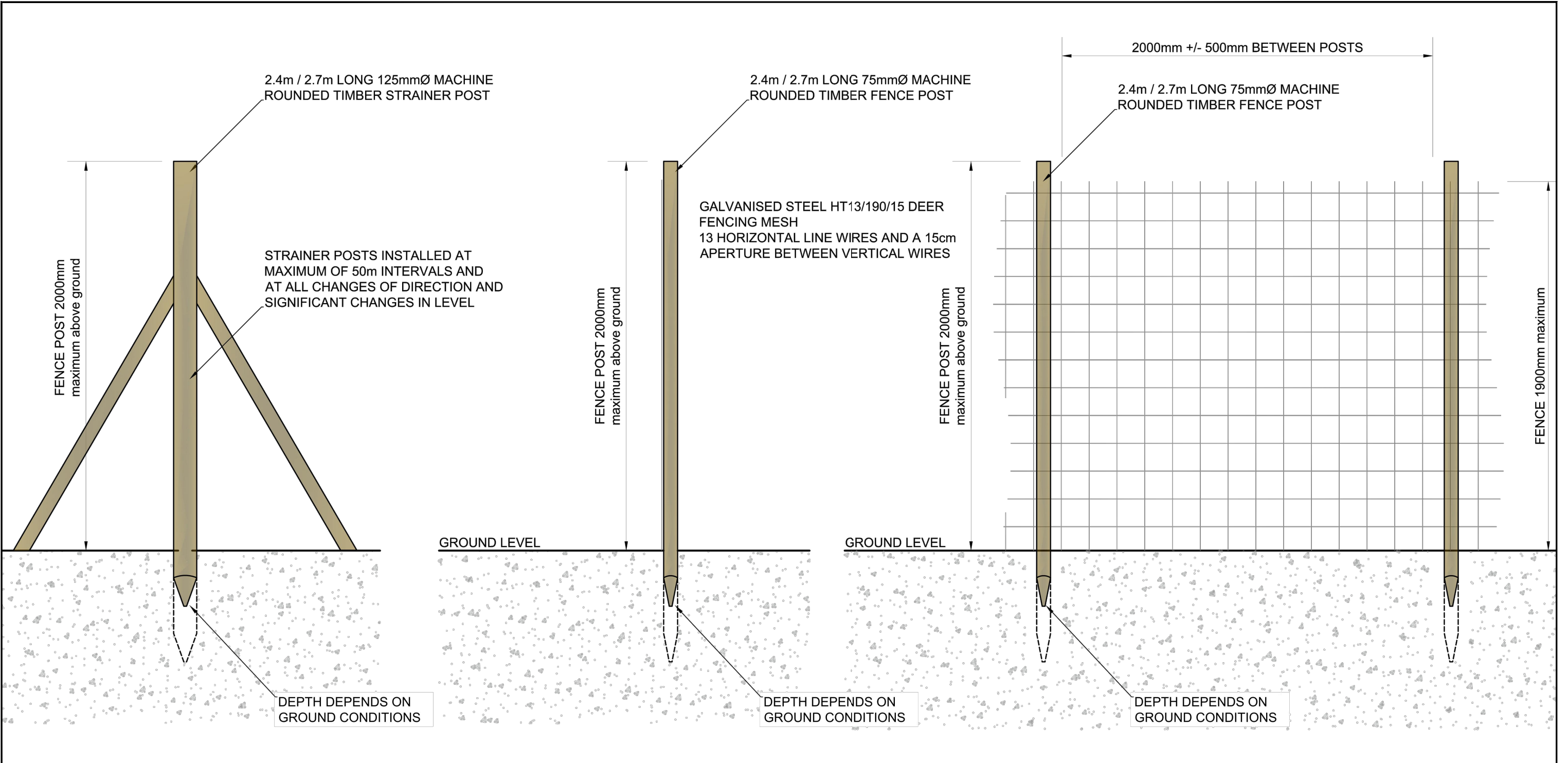
STRAINING POST
