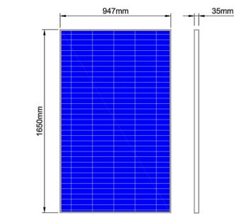
INDIVIDUAL PV PANEL DIMENSIONS
