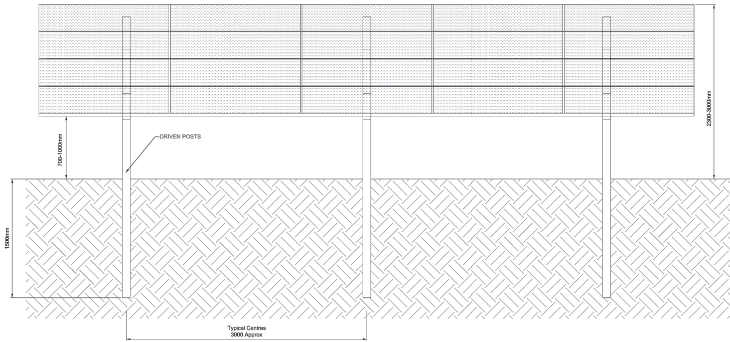
REAR VIEW OF PV PANEL INSTALLATION
