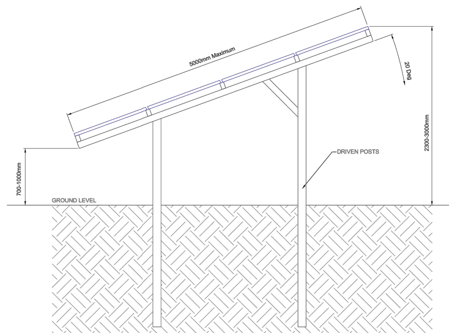
SIDE VIEW OF PV PANEL
